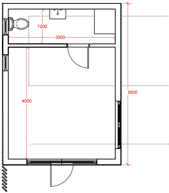
1 Proposed Ground Floor Plan 1:50
