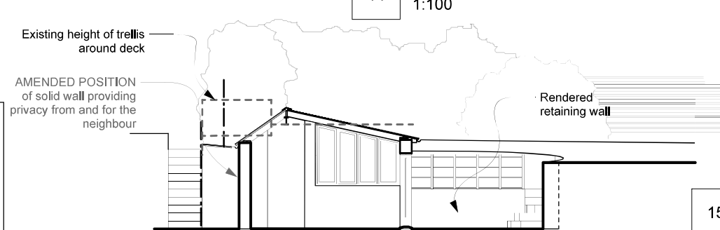
14 Proposed North Elevation 1:100
