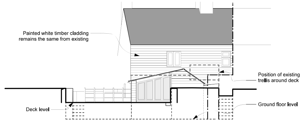
12 FF Proposed Rear Elevation 1:100
