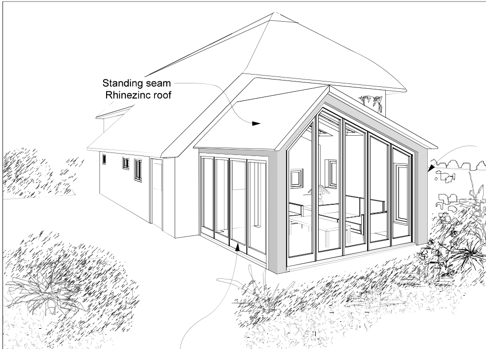
16 Proposed perspective from garden
